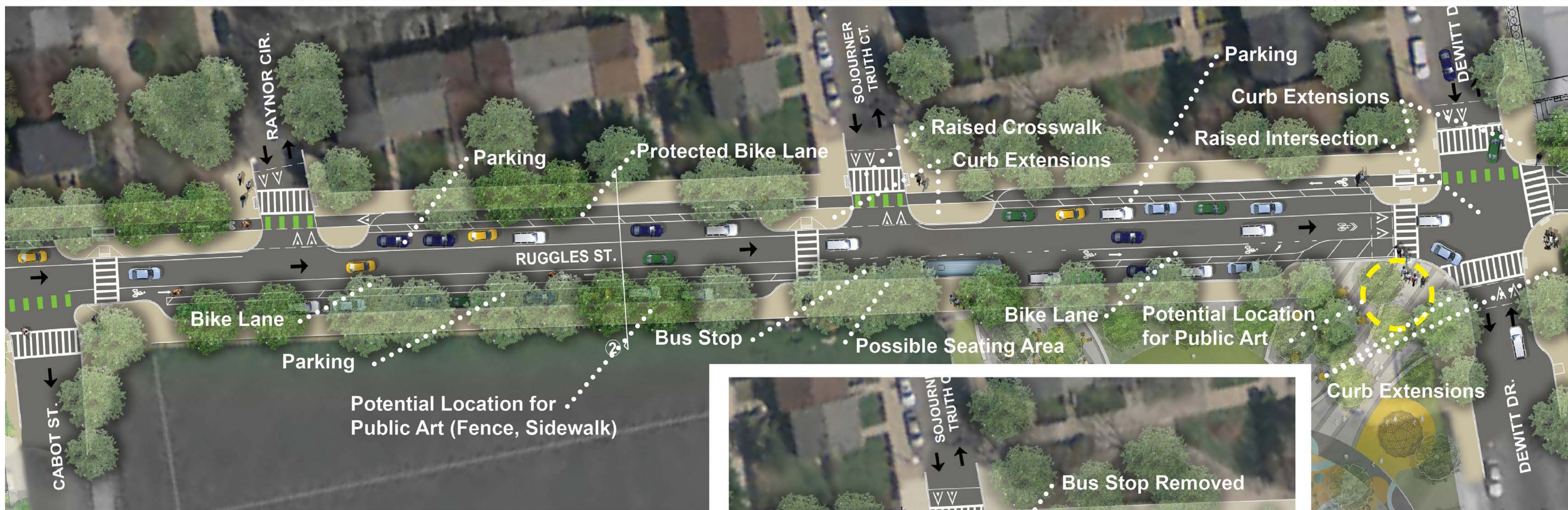
Preferred Option: Plan
