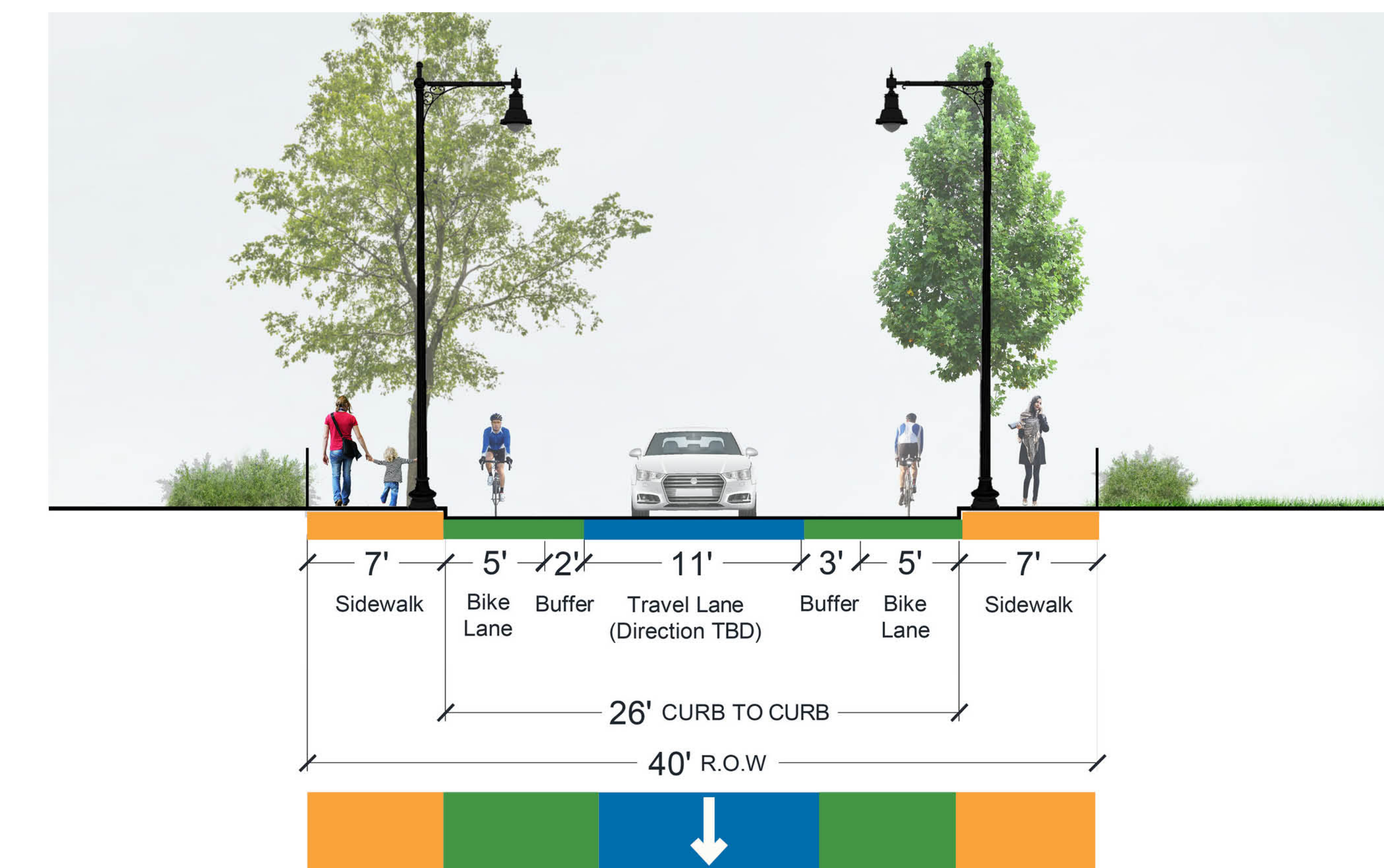
Preferred Option: Section
