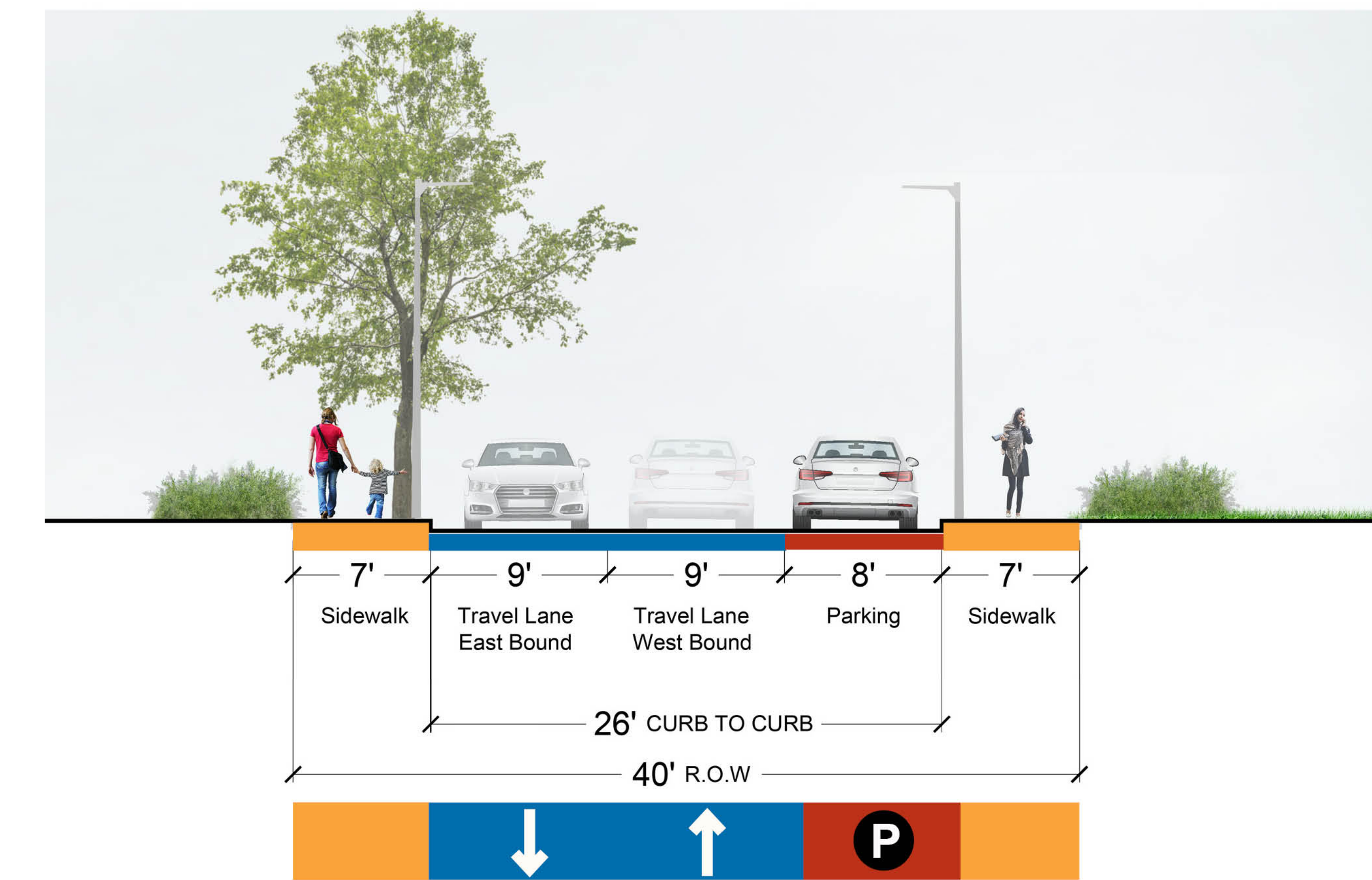
Existing Conditions: Section
