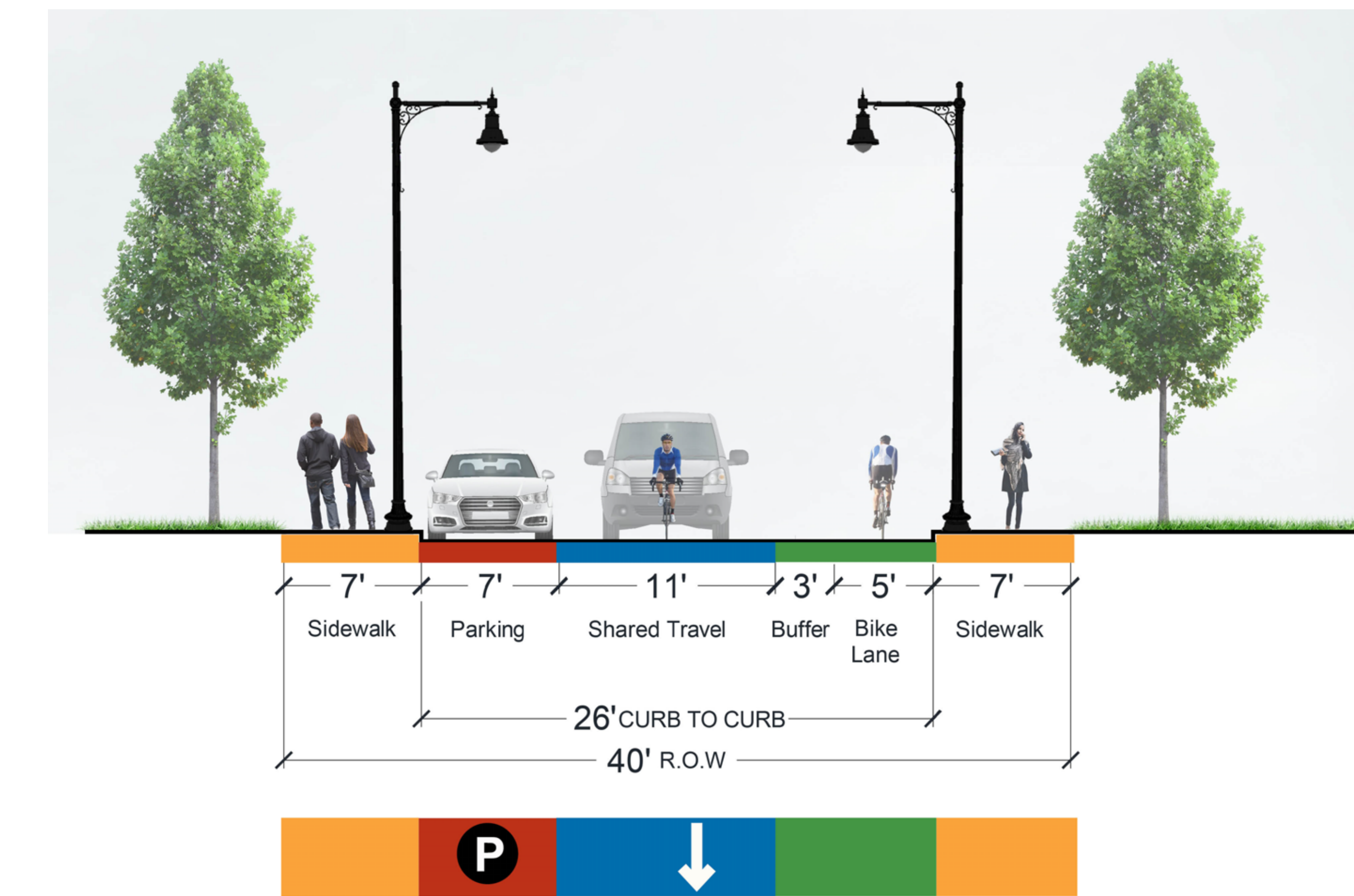
Preferred Option: Section
