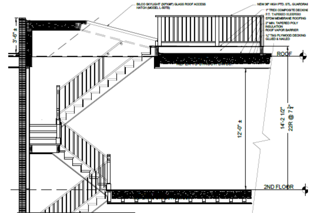
PROPOSED SECTION THROUGH ROOF HATCH
