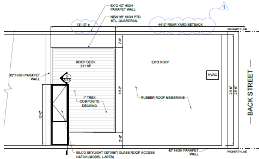
PROPOSED ROOF DECK PLAN
