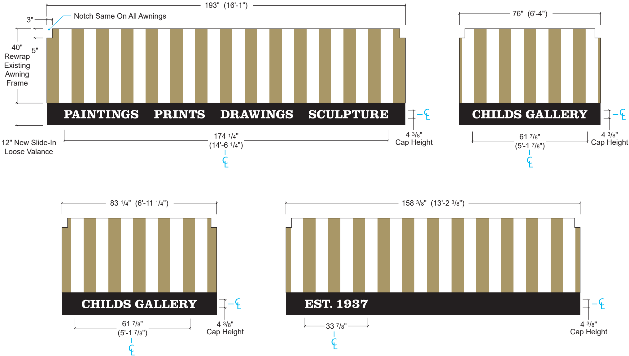
E1 Elevation: Awning Rewrap & New Valance Scale: 3/8" = 1'
