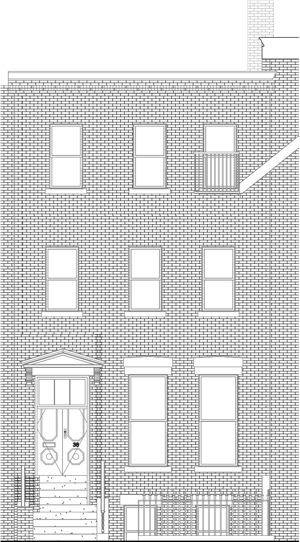
1 FRONT ELEVATION - EXISTING 1/8" = 1'-0"
