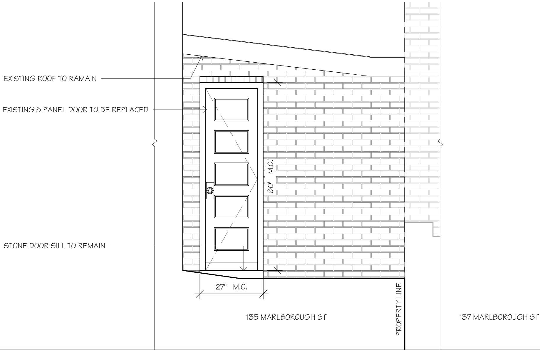
① Existing Bike Storage Elevation Looking South 1/2" = 1'-0"
