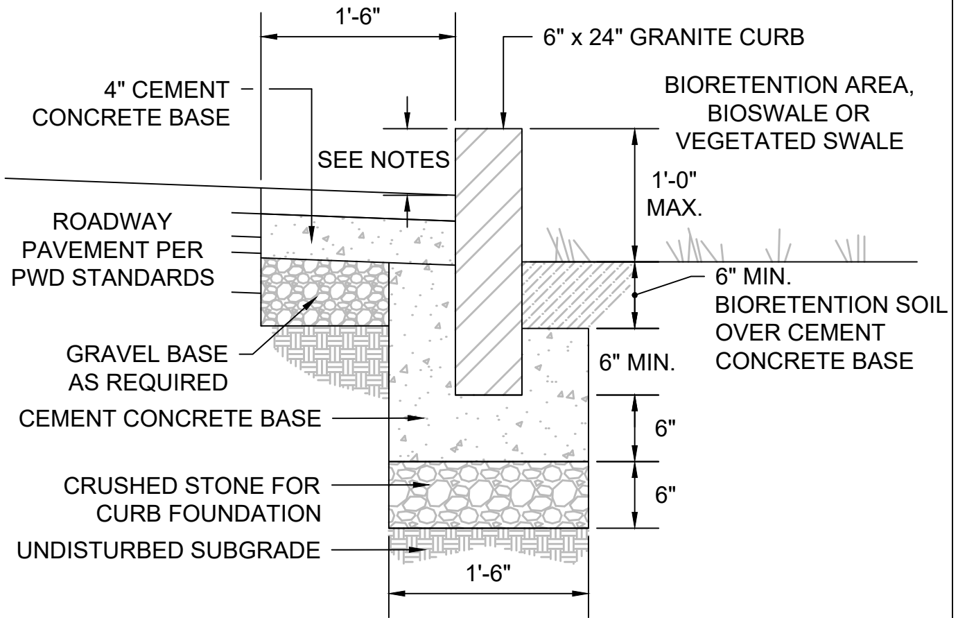
SECTION
