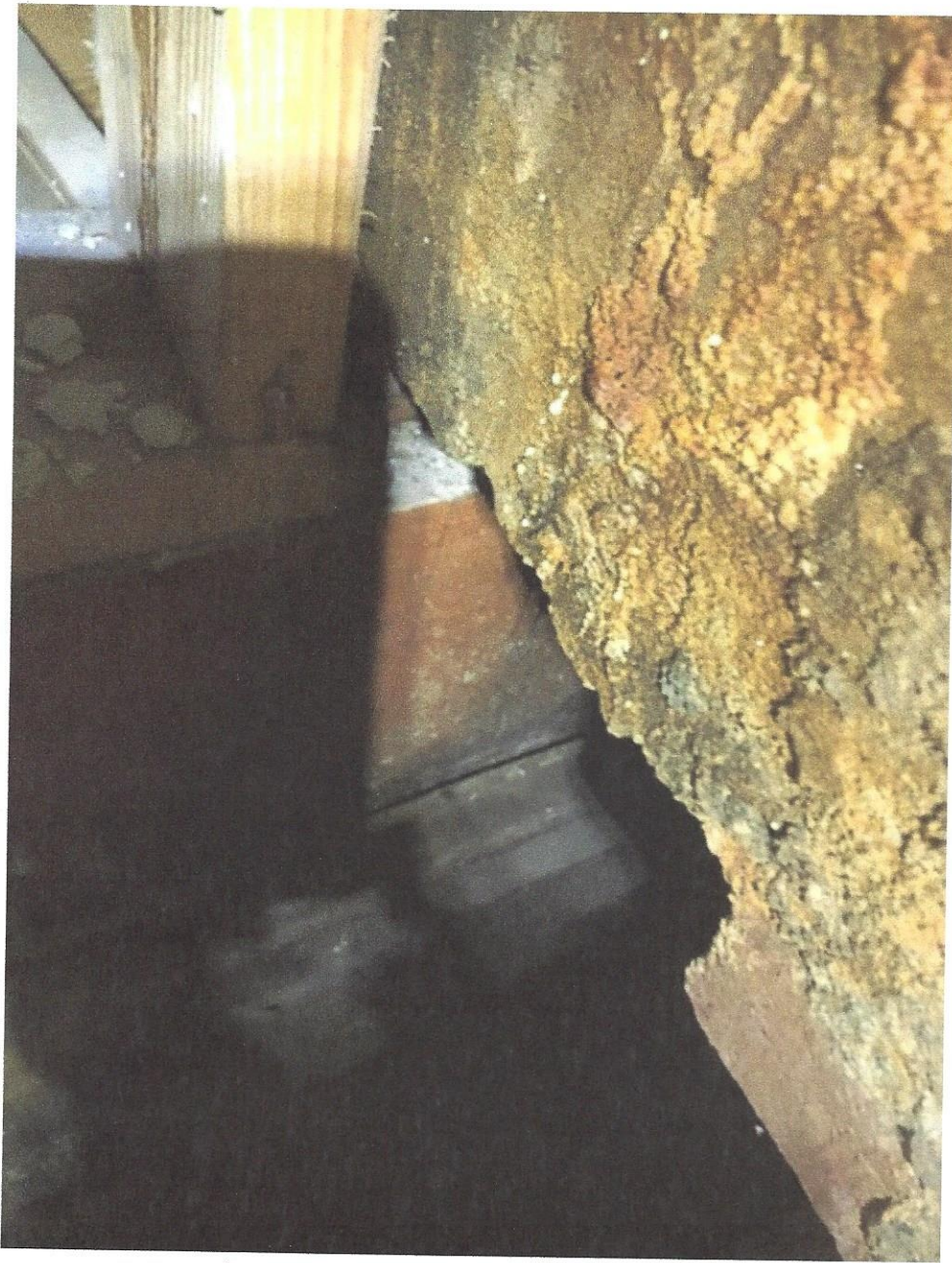
Corrosion of the Mortar at Bricks of chimney
