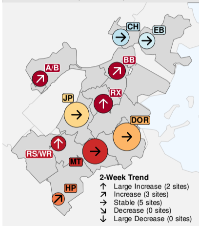
COVID-19 Wastewater Levels & Trends (17-Jul-2024)
