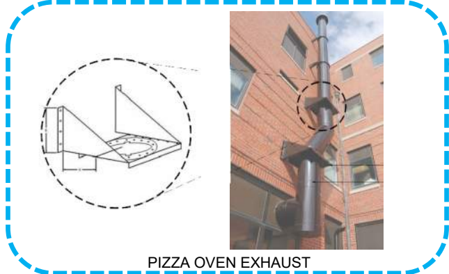
DUCT SUPPORT
