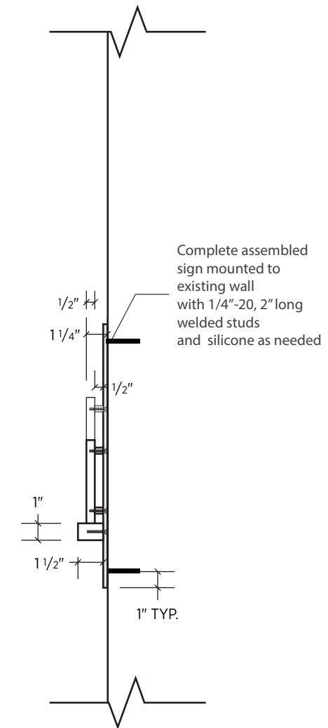
02 SIDE VIEW 1 1/2" = 1'-0"
