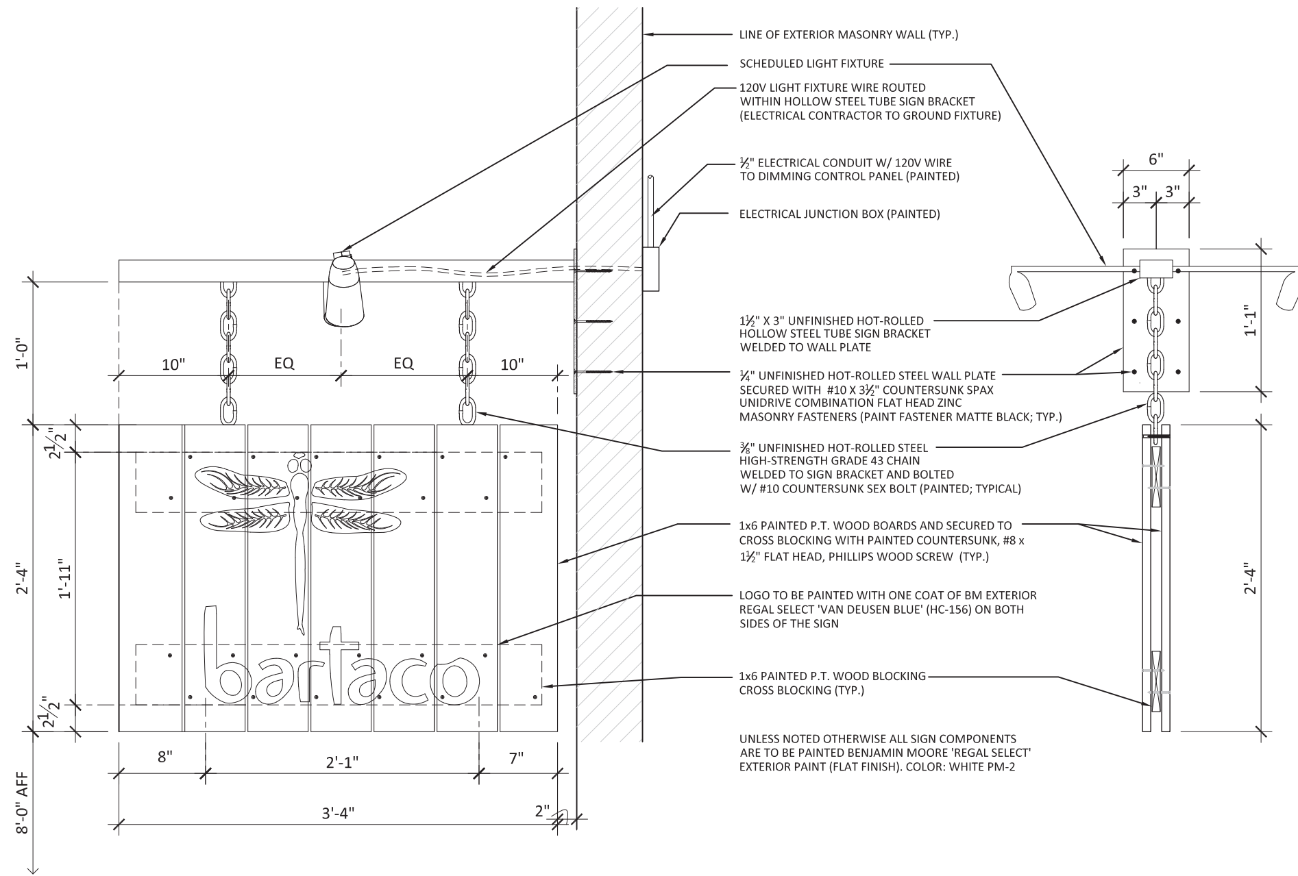
1 BLADE SIGN MOUNTING DETAIL 1" = 1'-0"
