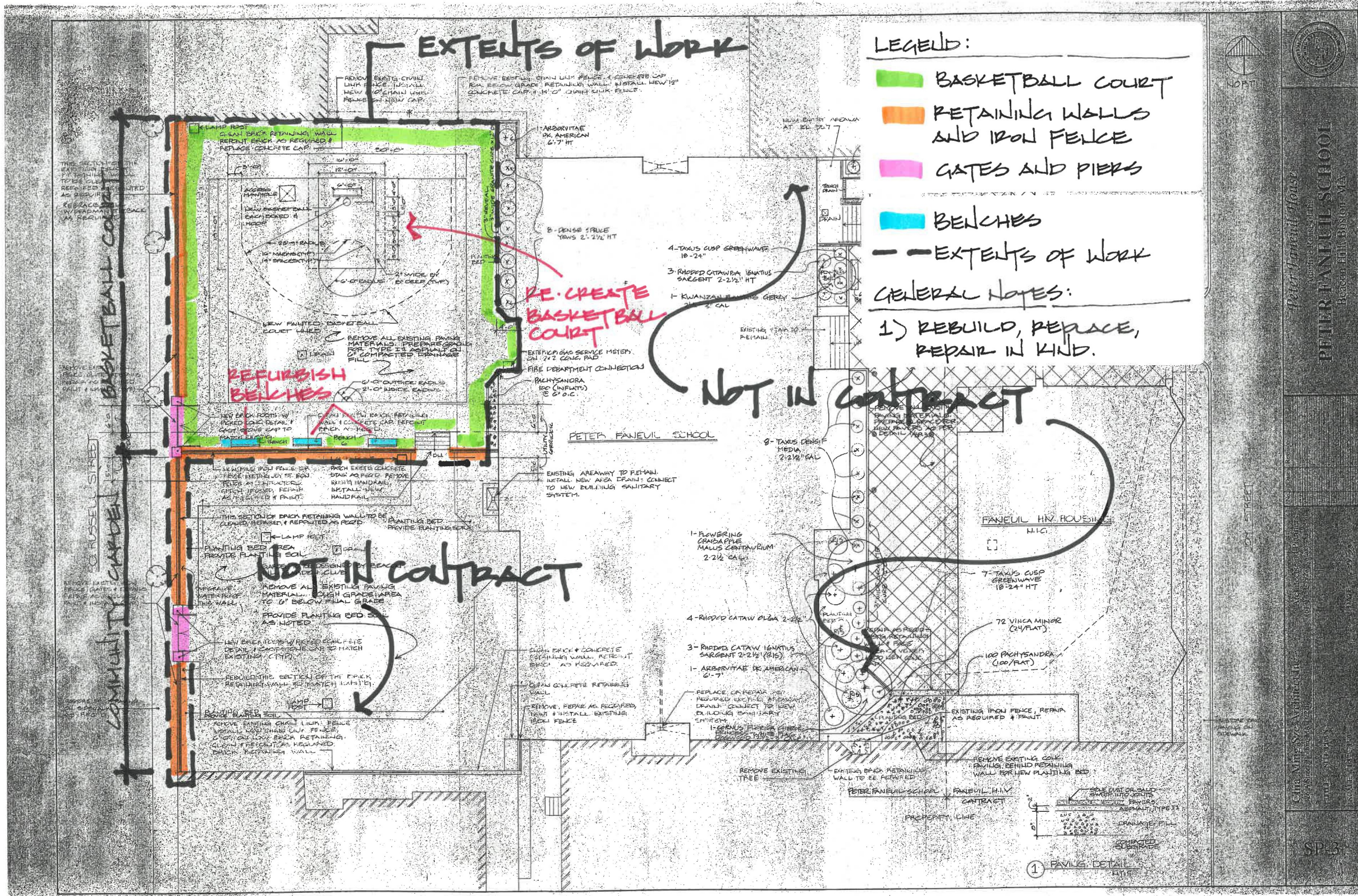
Site Plan
