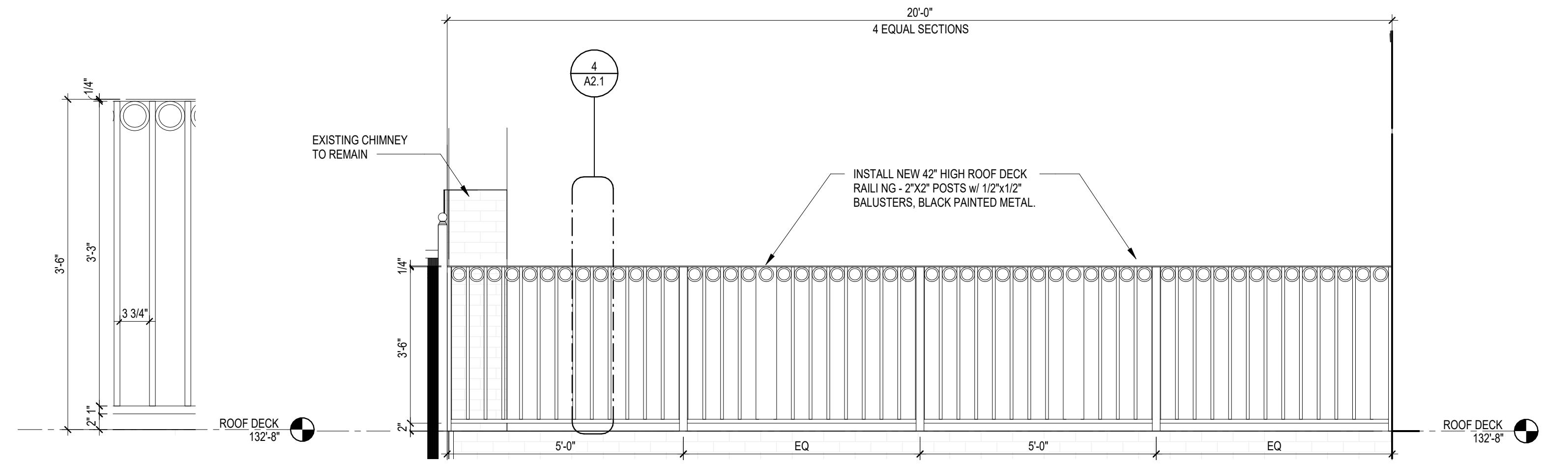
4 DECK RAILING ELEVATION - DETAIL 1" = 1'-0"
