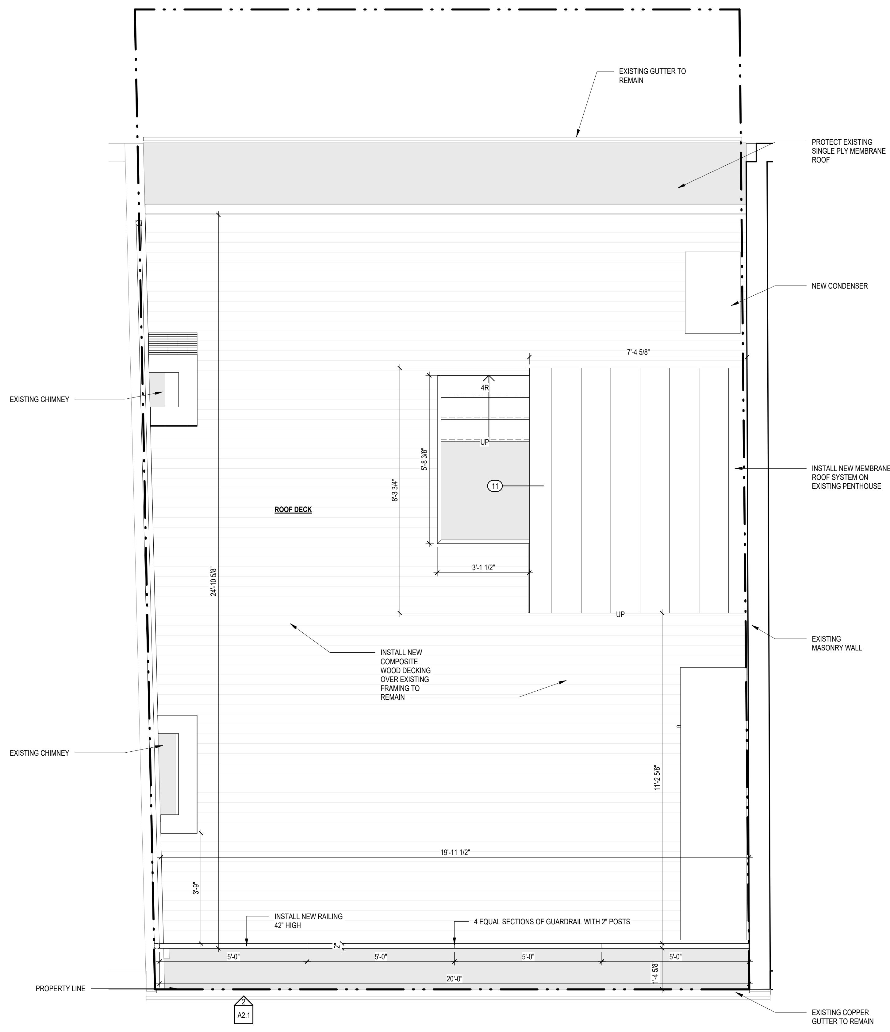
3 ROOF PLAN PROPOSED 1/2" = 1'-0"
