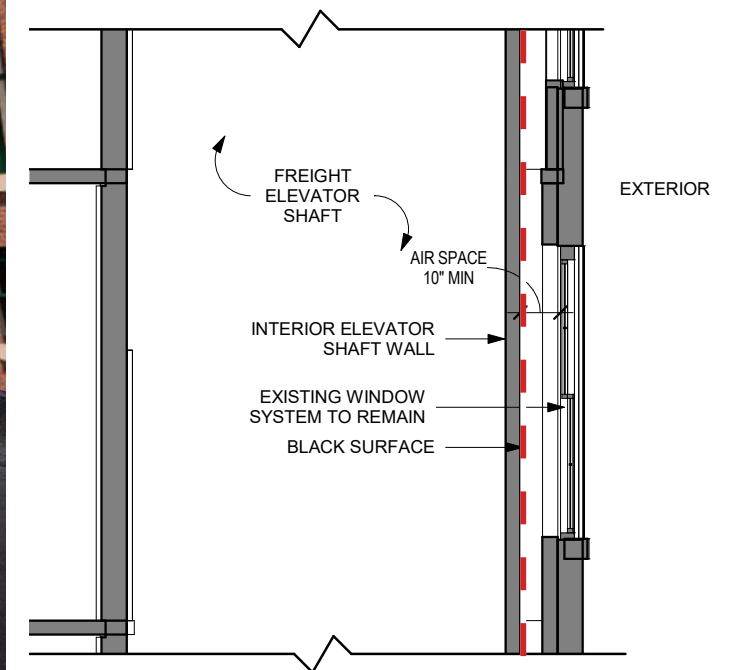
TYPICAL WALL SECTION AT FREIGHT ELEVATOR
