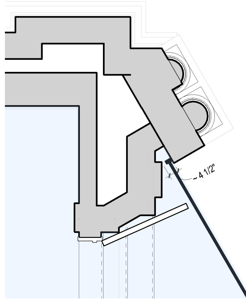
PLAN - PROPOSED
