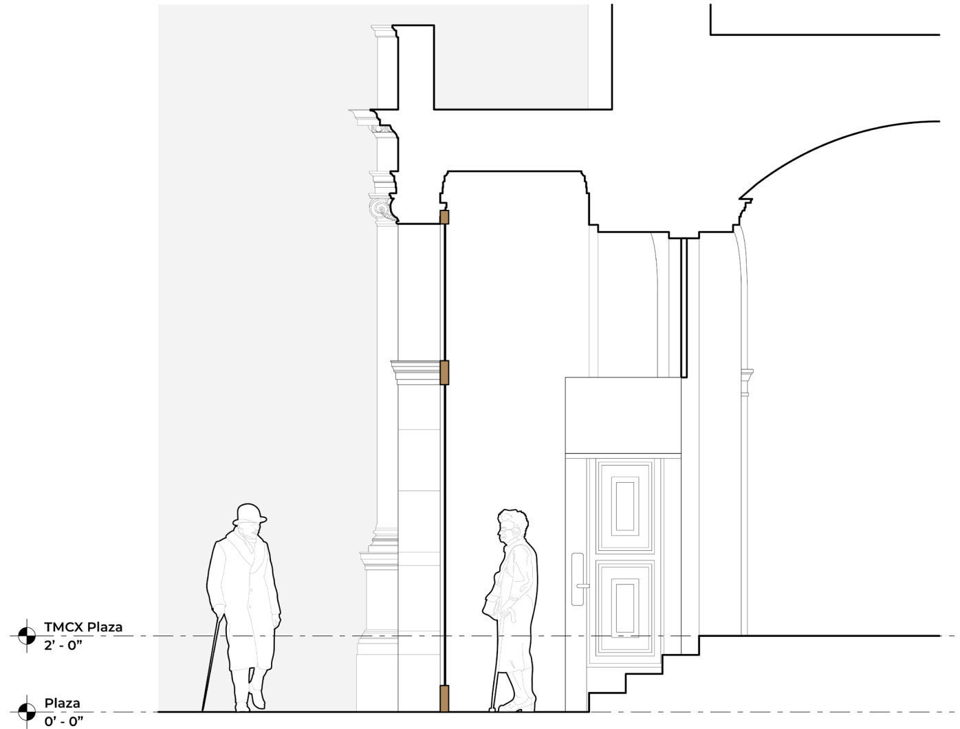
SECTION - PROPOSED
