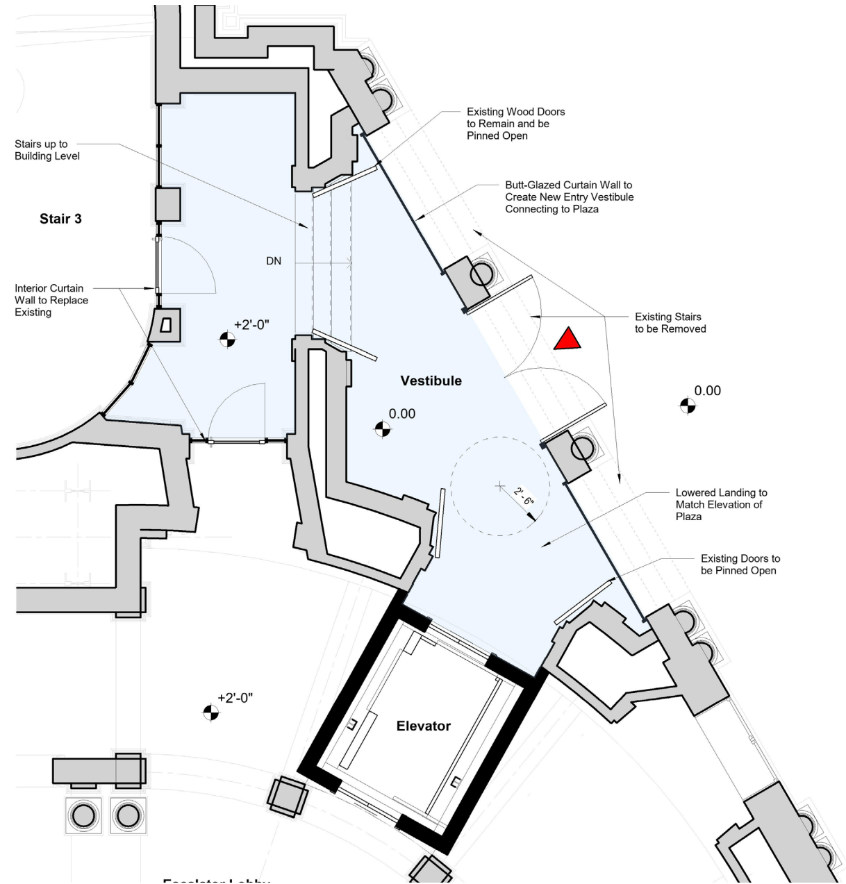
PLAN - PROPOSED
