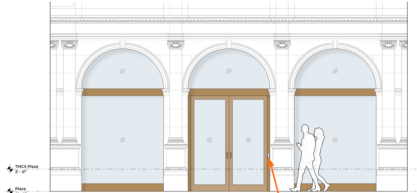
EXTERIOR ELEVATION - PROPOSED
