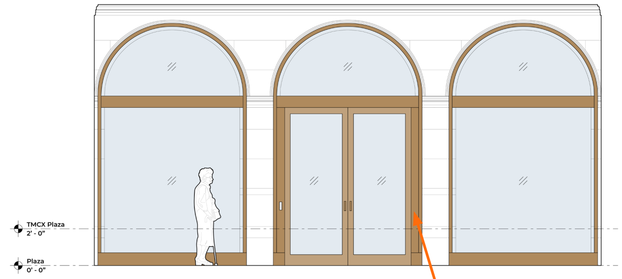
INTERIOR ELEVATION - PROPOSED
