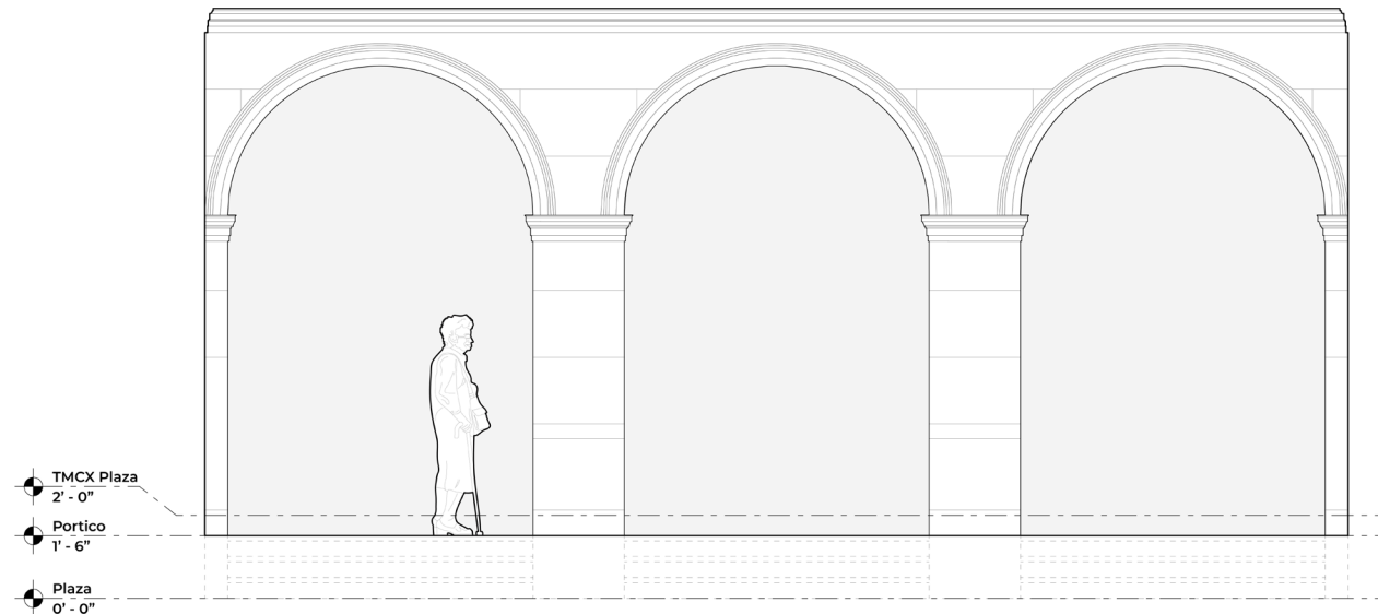
INTERIOR ELEVATION - EXISTING
