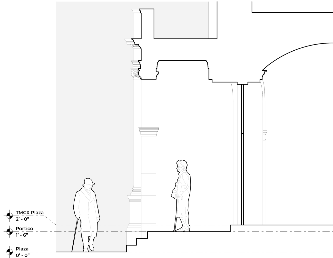
SECTION - EXISTING
