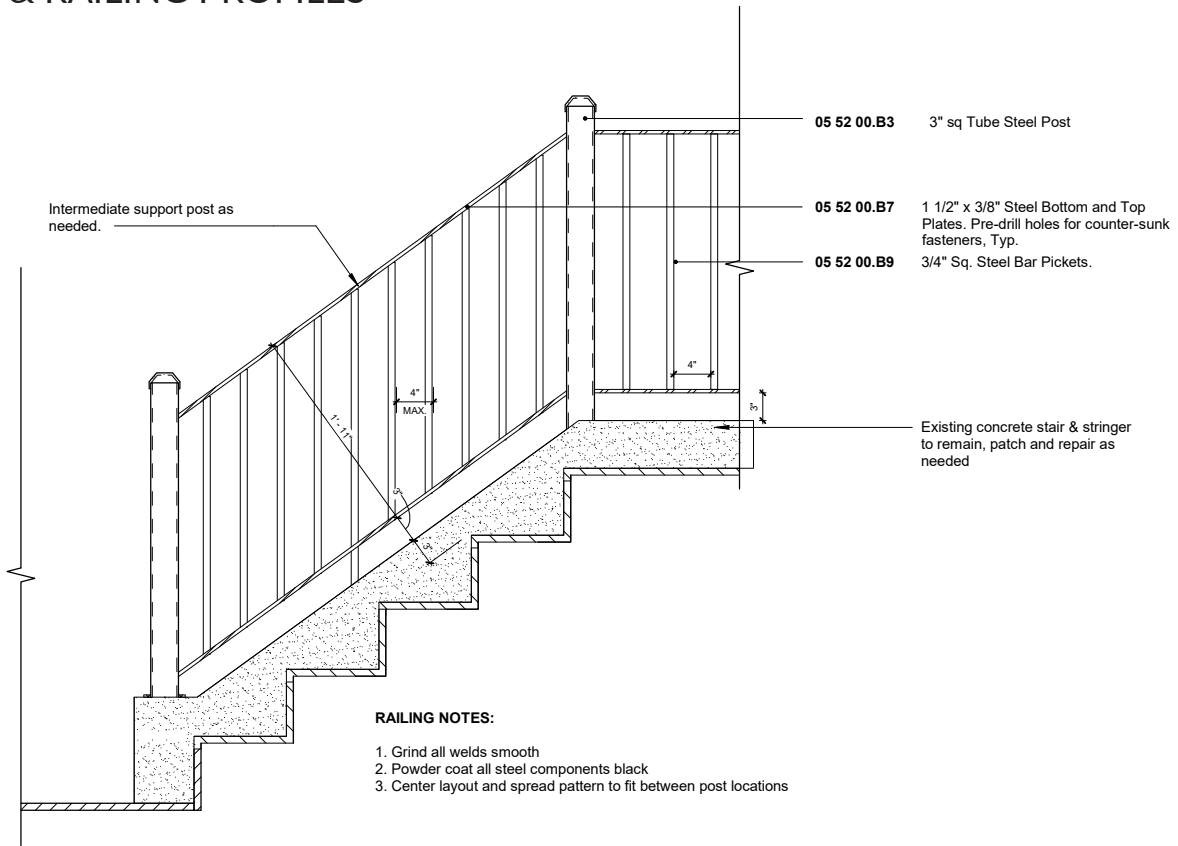
PROPOSED RAILING PROFILE @ FRONT STEPS
