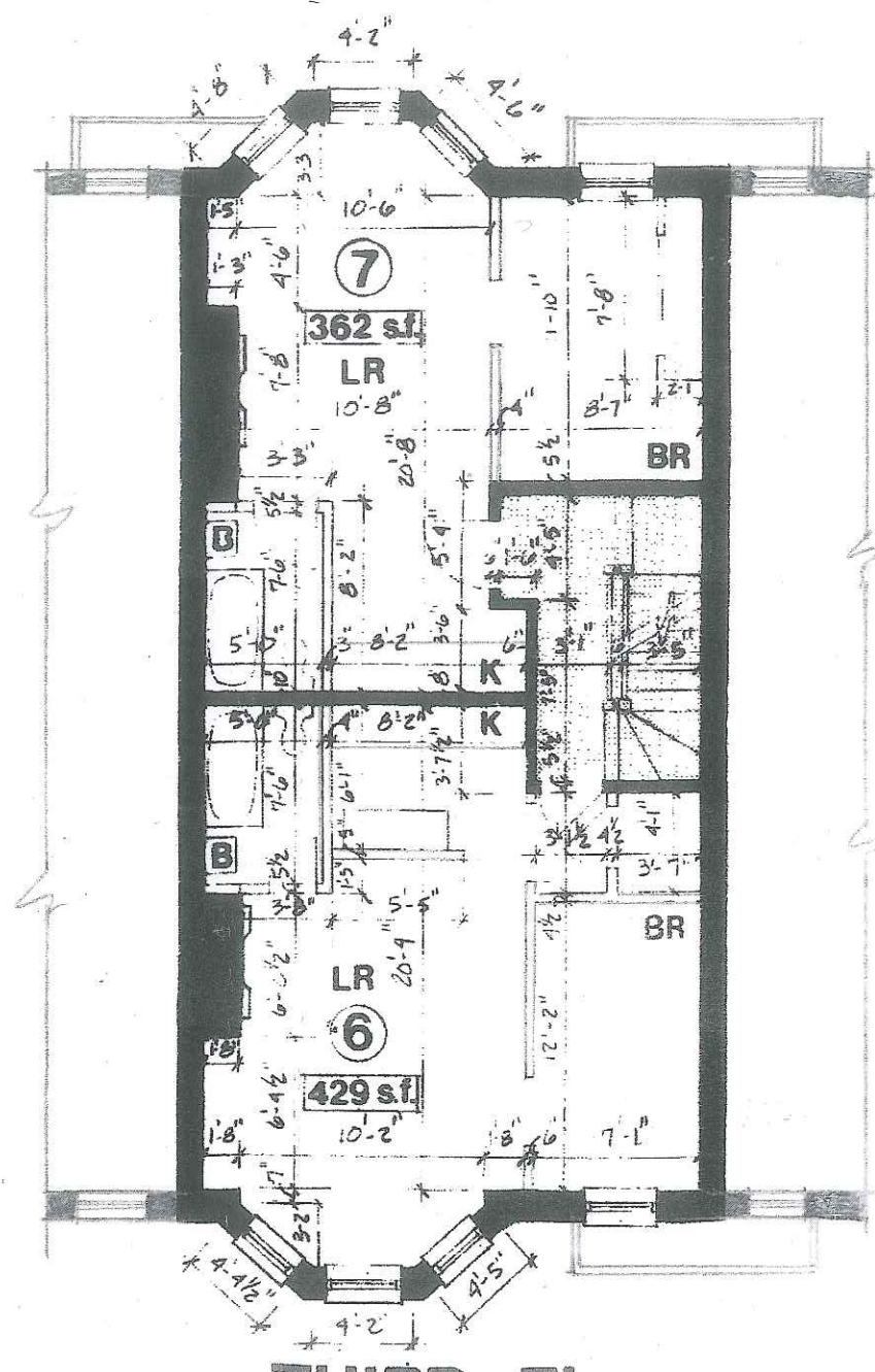
THIRD FL.
