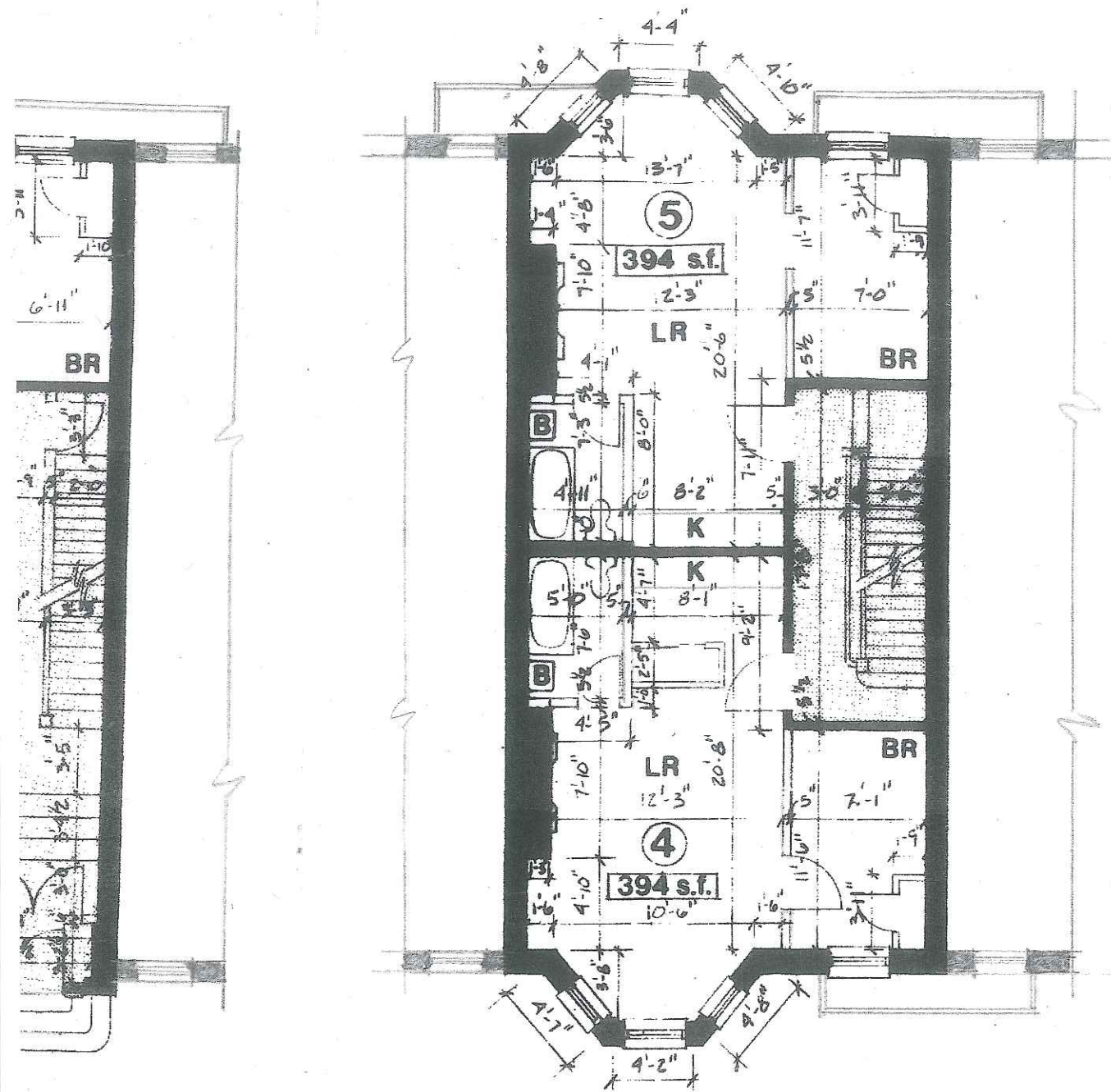
SECOND FL.
