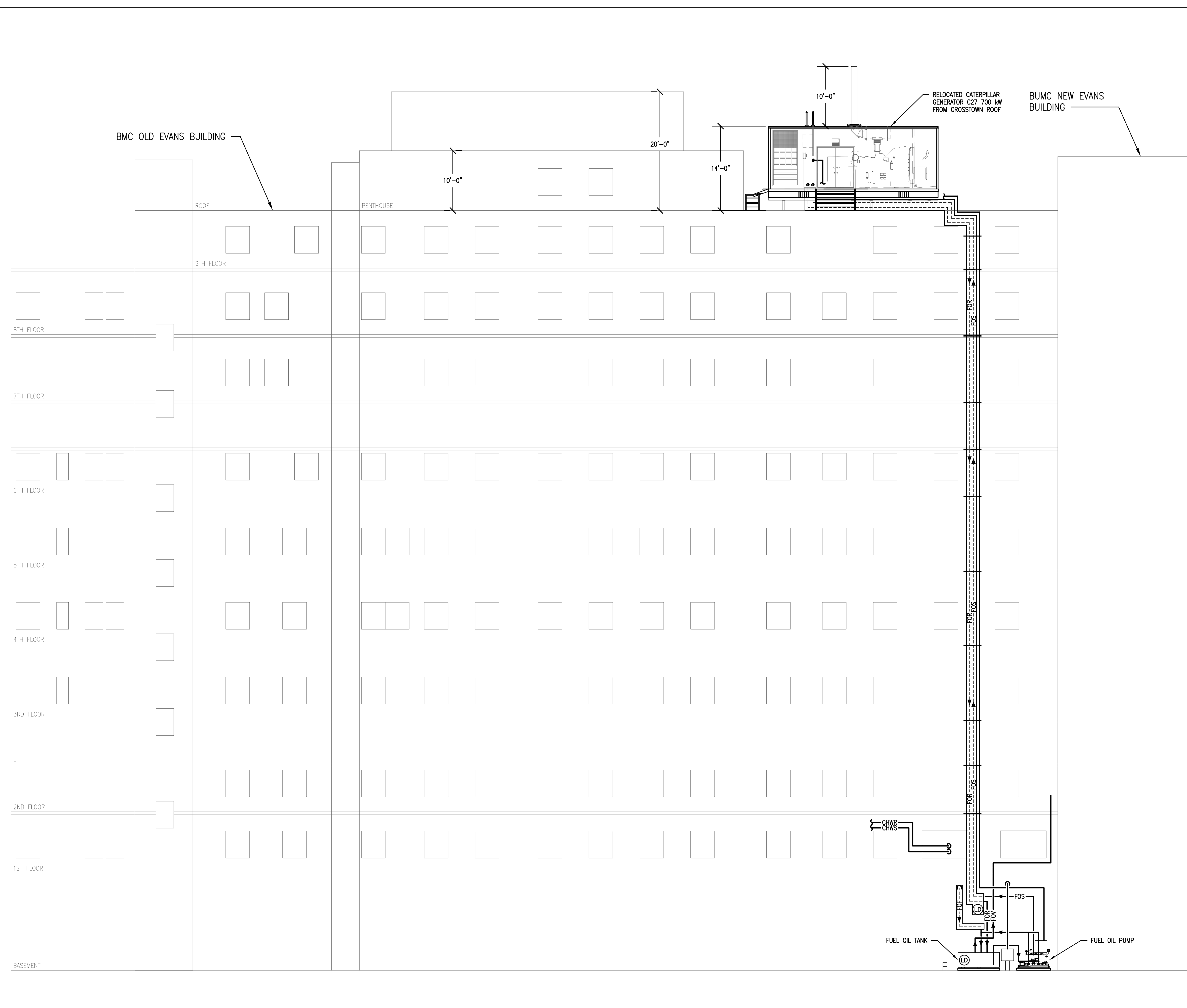
1 OLD EVANS FUEL OIL FLOW DIAGRAM – COURTYARD SIDE SCALE: NTS
