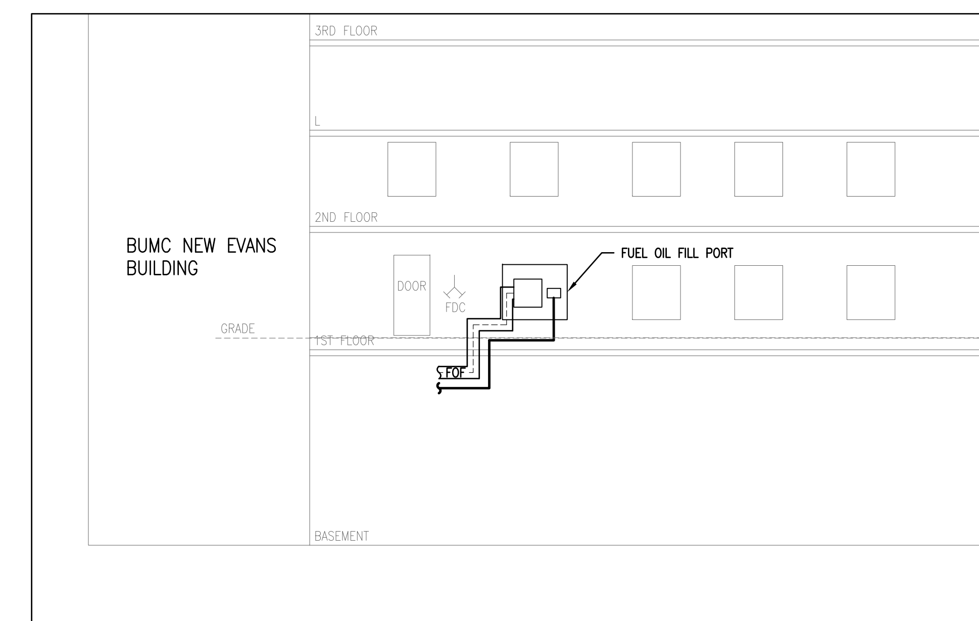
2 REMOTE FILL PORT – E. NEWTON STREET VIEW SCALE: NTS
