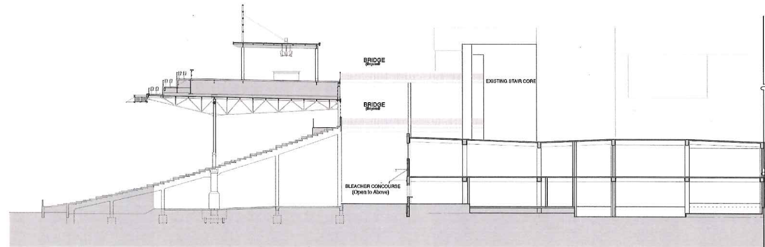
3 SECTION THRU RF ROOF PAVILION
