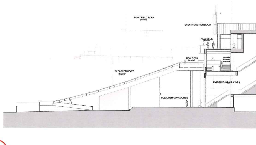
2 SECTION THRU STAIR CORE
