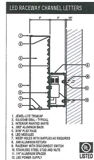
Side View Face lit channel letters
