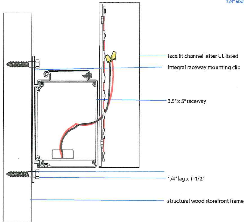
ST-1 Face lit channel letters - raceway wall mounted
