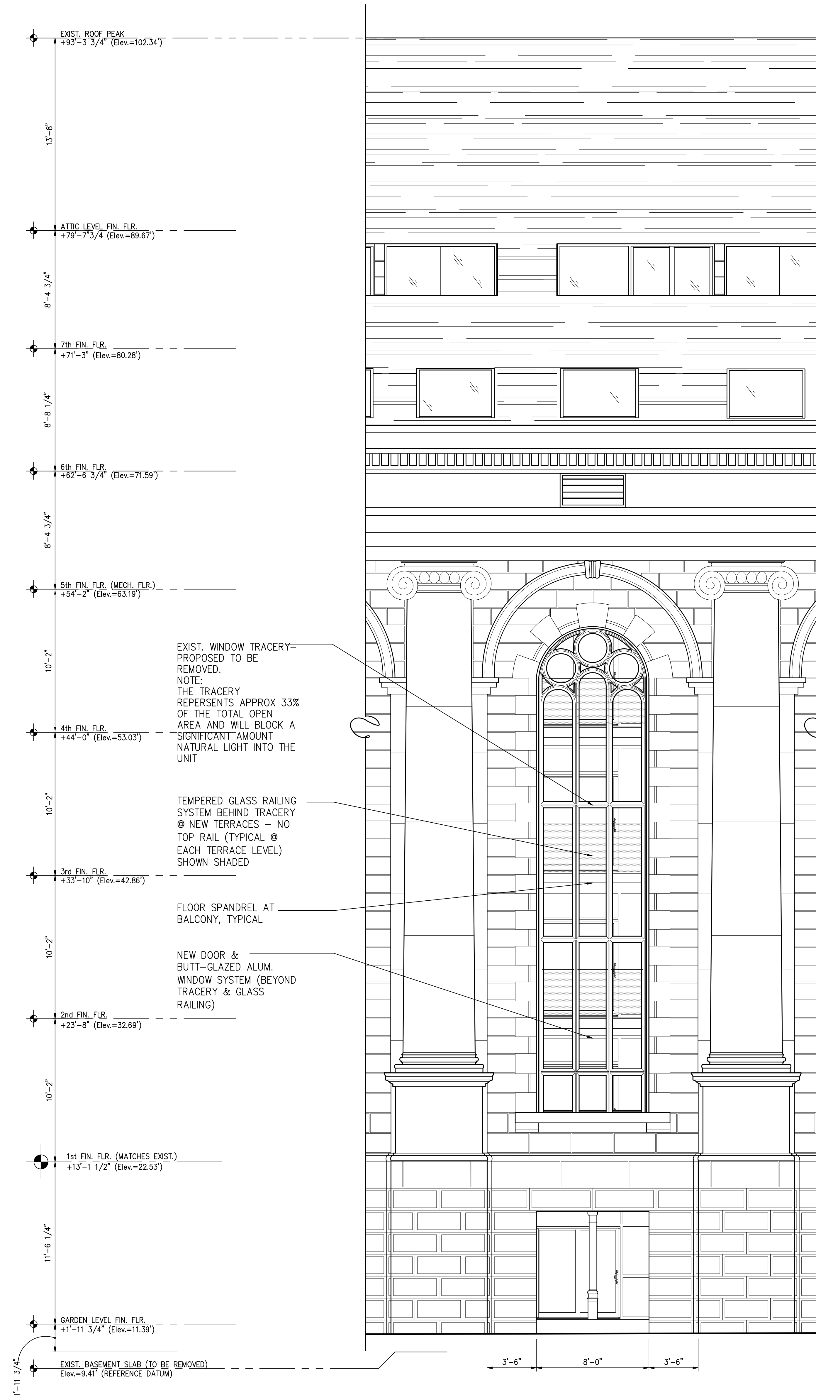
2 WINDOW ELEVATION w/TRACERY SCALE: 1/4" = 1'-0"
