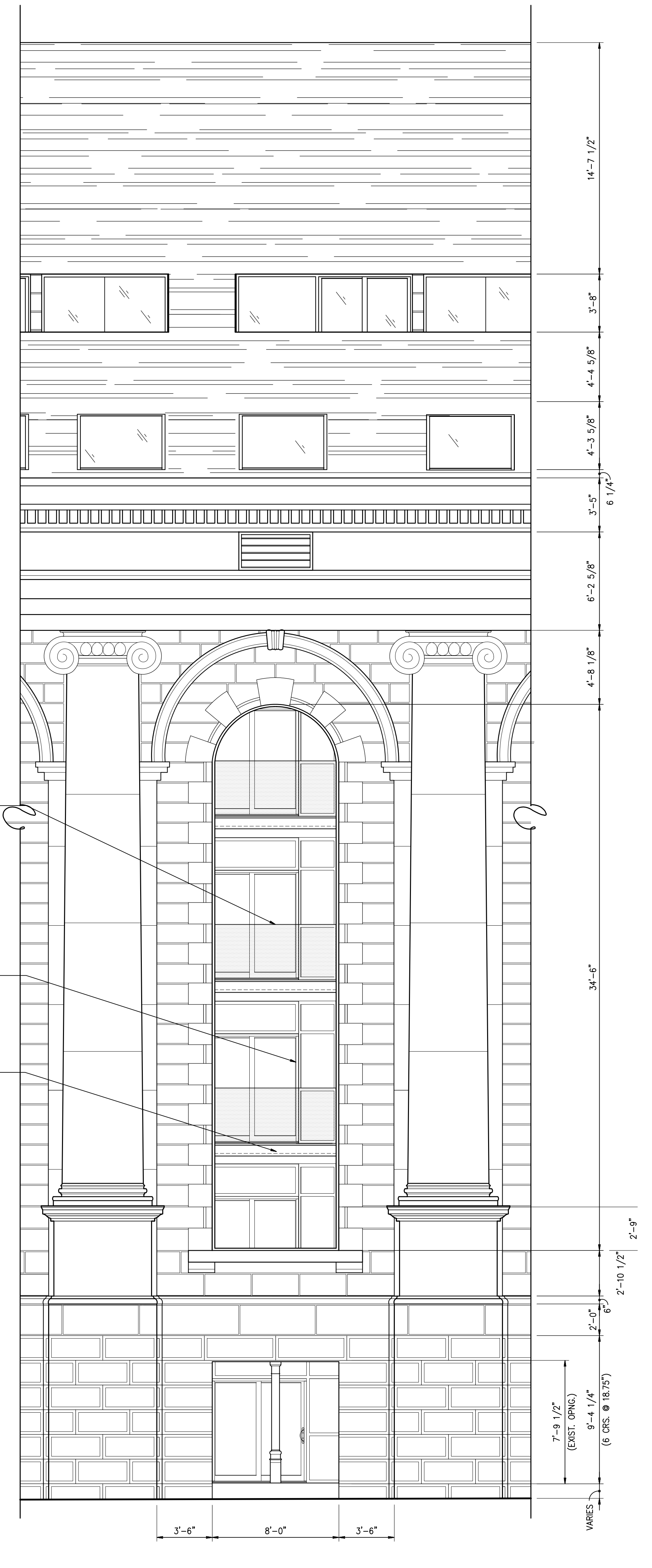
1 PROPOSED CHANGE TO WINDOW ELEVATION w/o TRACERY SCALE: 1/4" = 1'-0"
