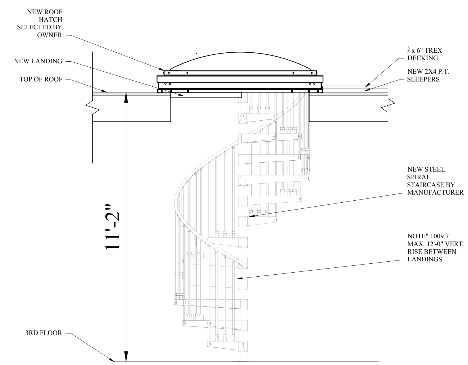
1 PROPOSED SPIRAL STAIR AND ROOF HATCH DETAIL 1/2" = 1'-0"
