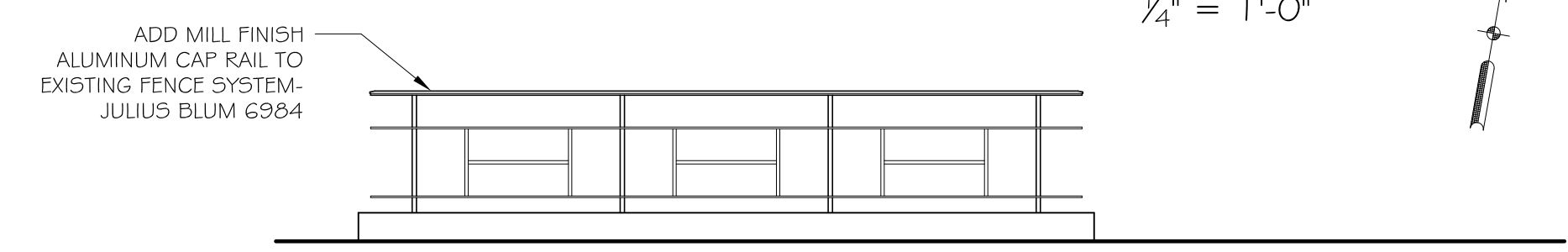
(E) RAIL @ SIDEWALK 1/4" = 1'-0"
